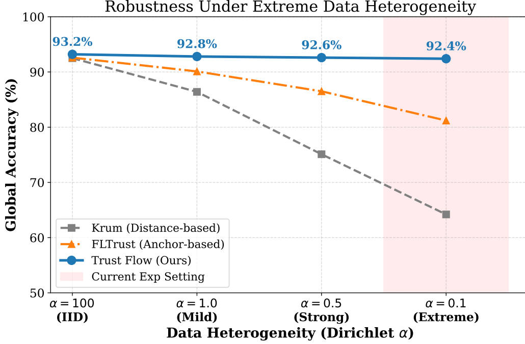
Figure 11: Robustness Stress Test under Varying Data Heterogeneity (Dirichlet \alpha )
